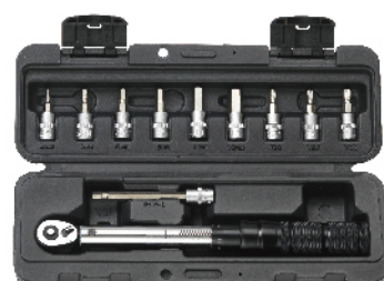
ST-A08 1/4" Drive torque wrench 2-14Nm , have 10pcs bit
